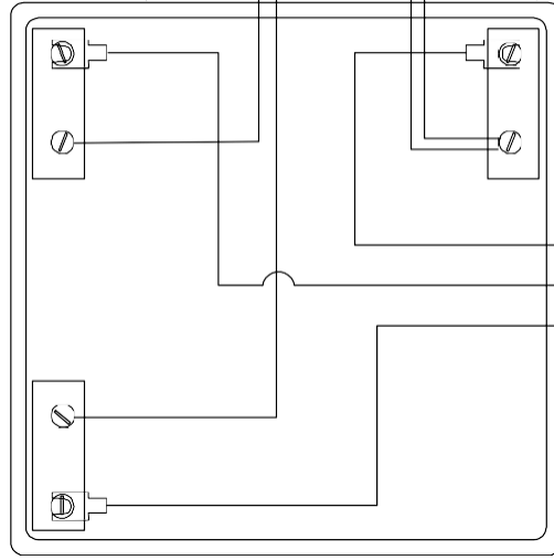
SR3T-P BUTON KASASI
